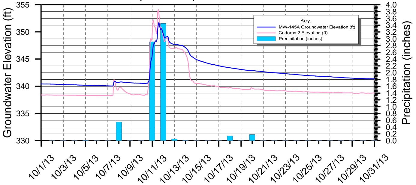
Figure 3.2-1 Water Level Response to Precipitation in Well MW-145A – October 2013
